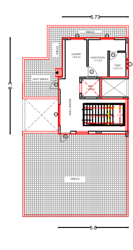
PRO. THIRD FLOOR PLAN.
