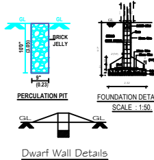
Dwarf Wall Details
