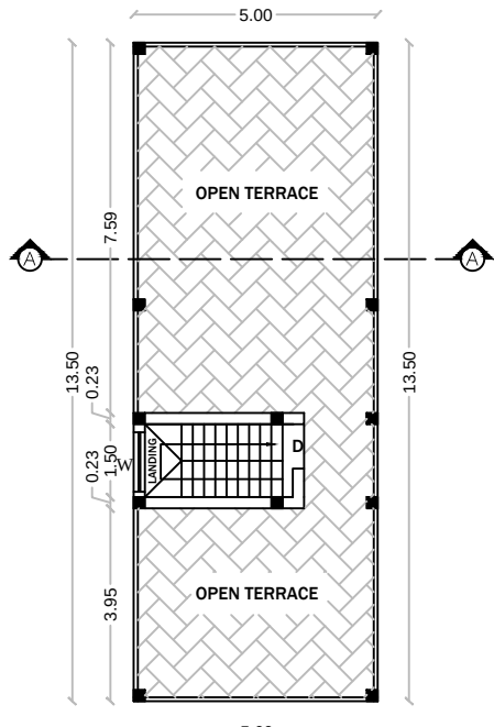
TERRACE FLOOR SCALE - 1:100
