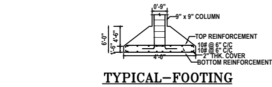
TYPICAL-FOOTING
