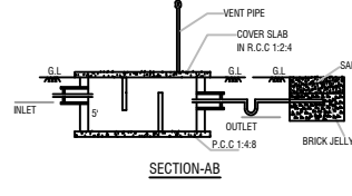
SECTION-AB
