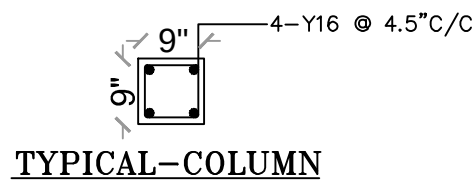
TYPICAL-COLUMN
