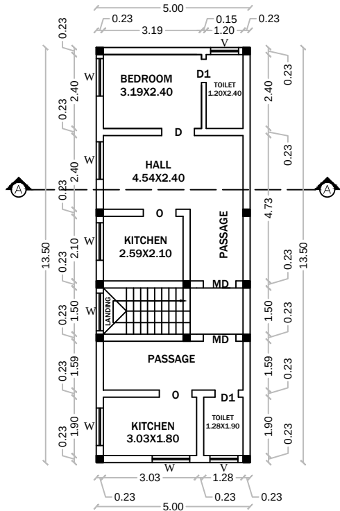
TYPICAL SECOND FLOOR & THIRD FLOOR SCALE - 1:100
