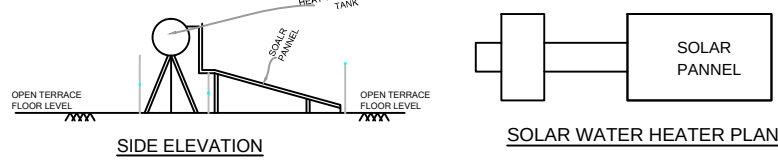
SIDE ELEVATION
