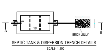
SEPTIC TANK & DISPERSION TRENCH DETAILS
