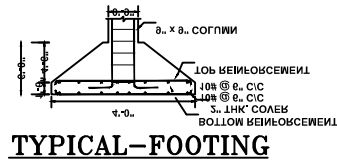
TYPICAL-FOOTING
