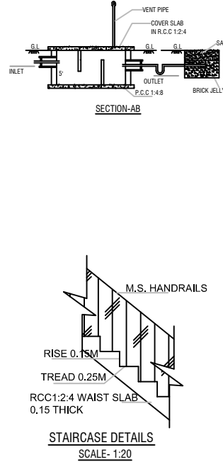
SCALE - 1:20
