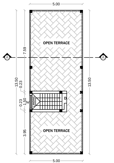
TERRACE FLOOR SCALE - 1:100
