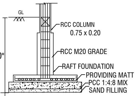
COLUMN FOOTING SCALE- 1:100
