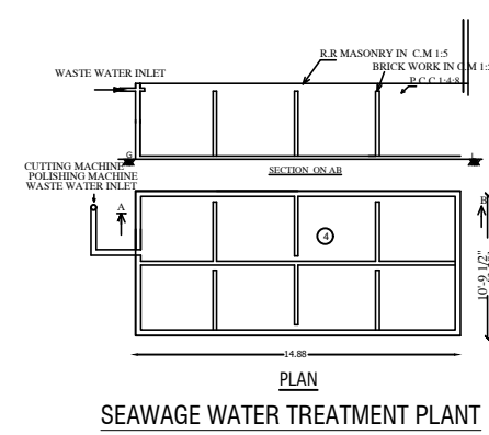
SEWAGE WATER TREATMENT PLANT
