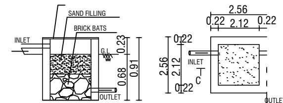
SECTION- CD RAIN WATER HARVESTING SYSTEM
