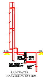
RAIN WATER HARVESTING SYSTEM
