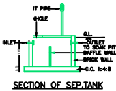
SECTION OF SEPTIC TANK
