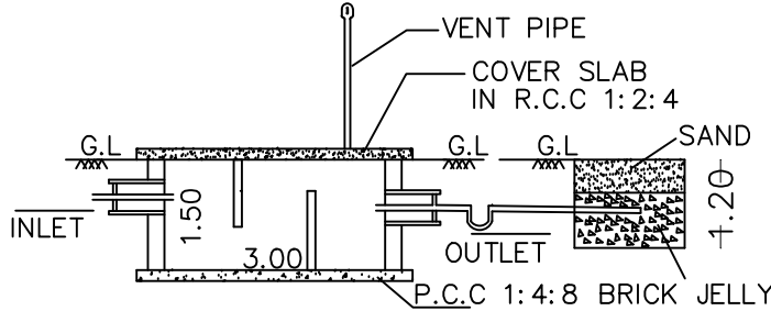
SECTION-AB
