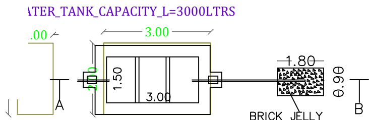
SEPTIC TANK & DISPERSION TRENCH DETAILS
