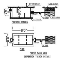
SEPTIC TANK AND DISPERSION TRENCH DETAILS
