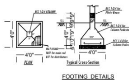
FOOTING DETAILS
