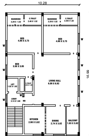
TYPICAL FIRST, SECOND & THIRD FLOOR PLAN
