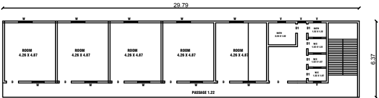
THIRD FLOOR
