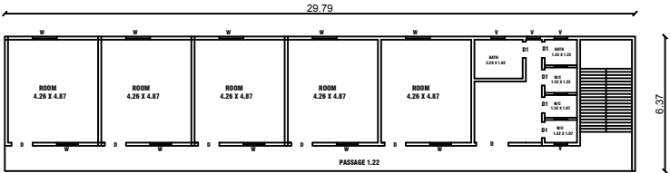
SECOND FLOOR
