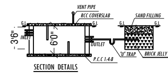
SECTION DETAILS
