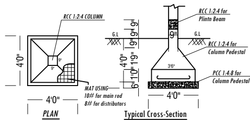
FOOTING DETAILS
