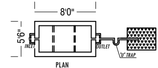
SEPTIC TANK AND DISPERSION TRENCH DETAILS
