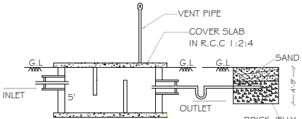
SECTION-AB
