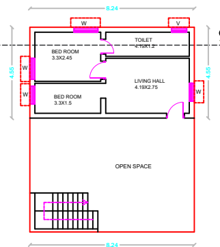
PRO. SECOND FLOOR PLAN SCALE:1:100
