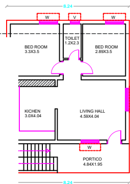
IRT'S FLOOR PLAN SCALE:1:100
