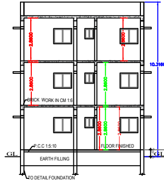
SECTION "A-B"
