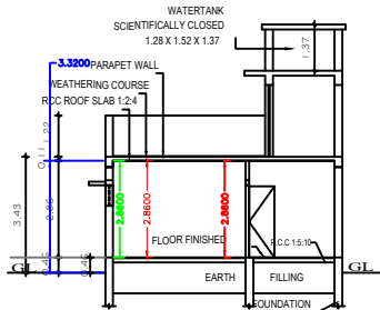
SECTION "A-B"
