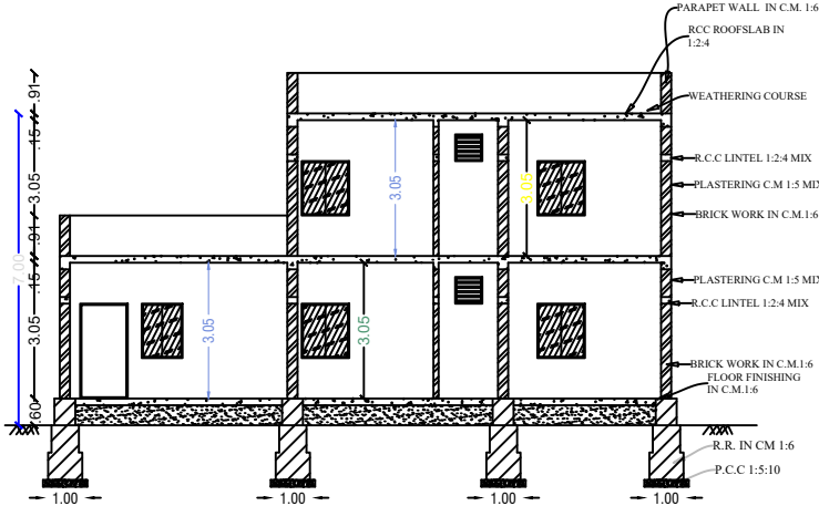
SECTION ON-"AB"
