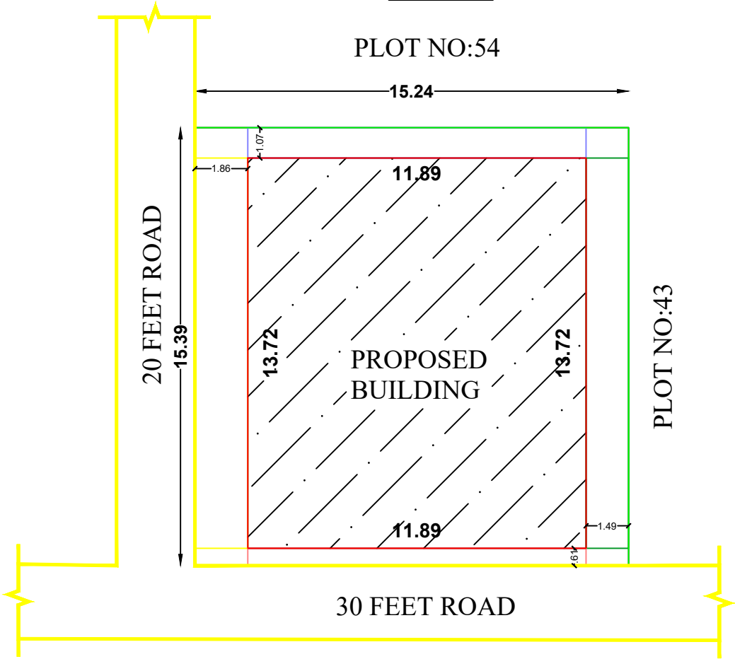
SITE PLAN
