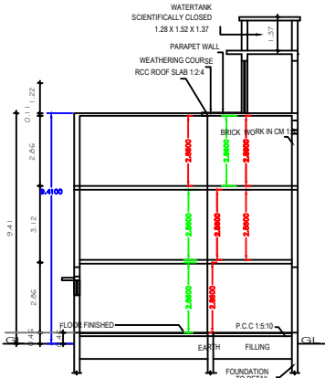
SECTION "A-B"
