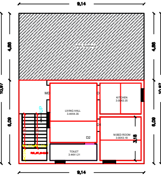
PRO. SECOND FLOOR PLAN.
