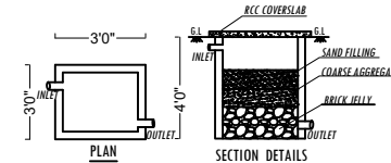
RAINWATER HARVESTING SYSTEM
