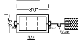
SEPTIC TANK AND DISPERSION TRENCH DETAILS
