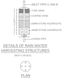
SECTION-AB
