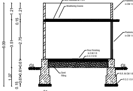
SECTION AT 'AA'
