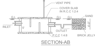
SECTION-AB
