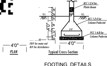
FOOTING DETAILS
