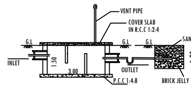
SECTION-AB
