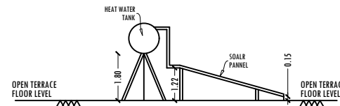
SIDE ELEVATION
