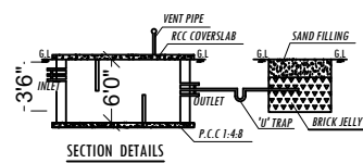
SECTION DETAILS
