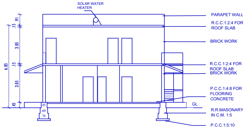
SECTION ON A
