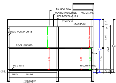
SECTION "A-B"
