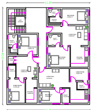
PRO. SECOND FLOOR PLAN.
