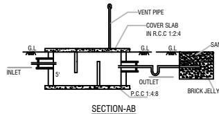
SECTION-A-B
