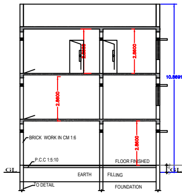
SECTION "A-B"
