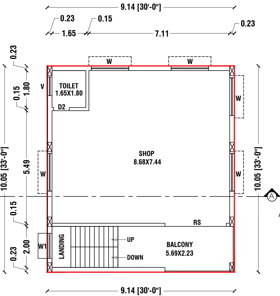
FRIST FLOOR PLAN
