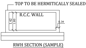
RWHP SECTION (SAMPLE)
