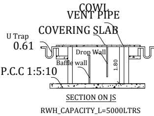
SECTION ON JS
