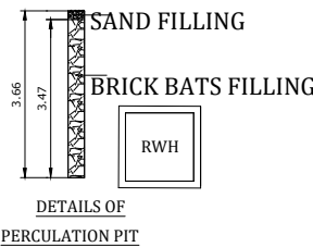
DETAILS OF PERCOLATION PIT
