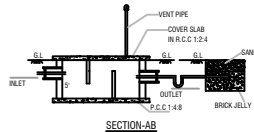
SECTION-AB
