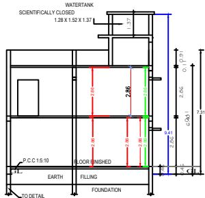
SECTION "A-B"
