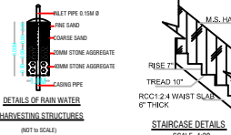
STAIRCASE DETAILS SCALE-1:20
