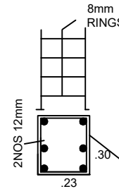
COLUMN DETAILS (NOT TO SCALE)
