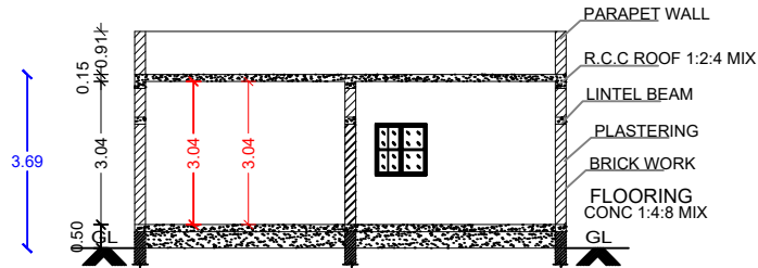
SECTION: A-B
