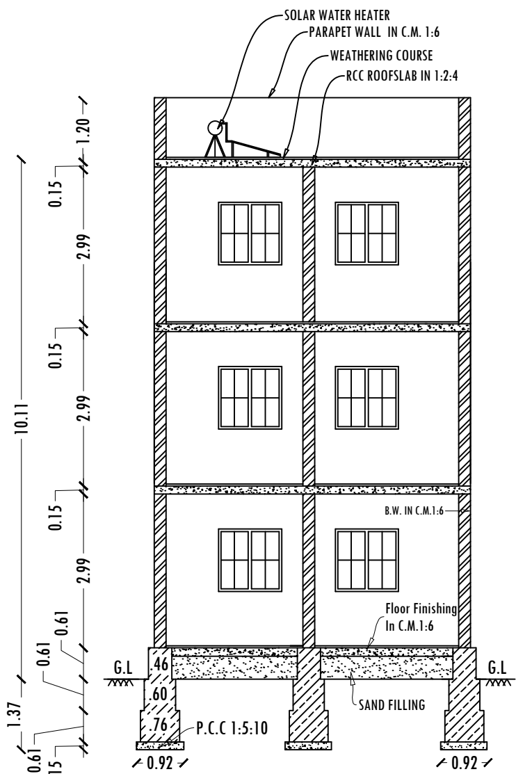
SECTION -AA
