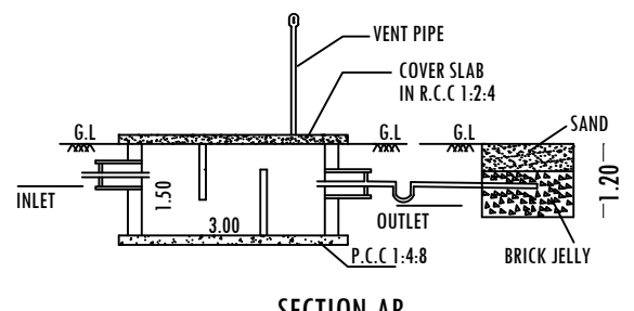
SECTION-AB
