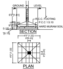
FOUNDATION DETAILS
