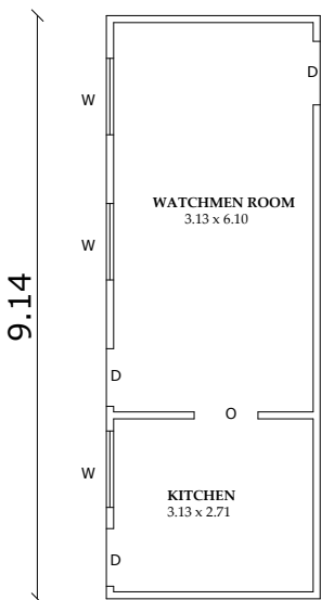
GROUND FLOOR - 2
