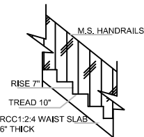
STAIRCASE DETAILS SCALE- 1:20
