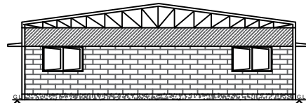
FRONT ELEVATION
