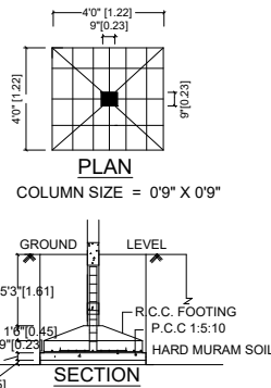
FOUNDATION DETAILS
