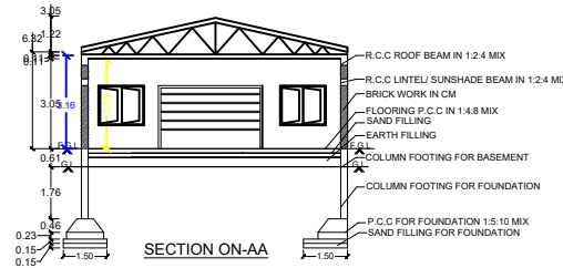
SECTION ON-AA
