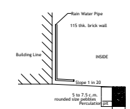
FOUNDATION DETAILS
