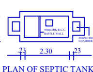
PLAN OF SEPTIC TANK
