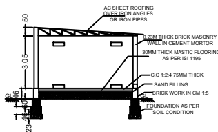
SECTION
