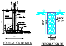
FOUNDATION DETAILS
