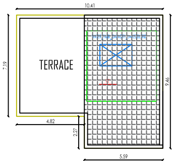
TERRACE FLOOR
