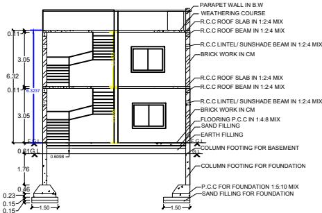
SECTION ON-AA
