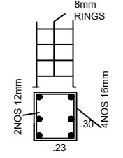
COLUMN DETAILS
