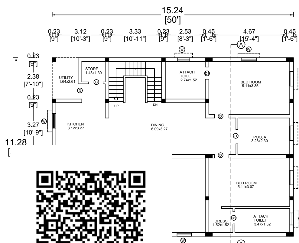
ND FLOOR PLAN
