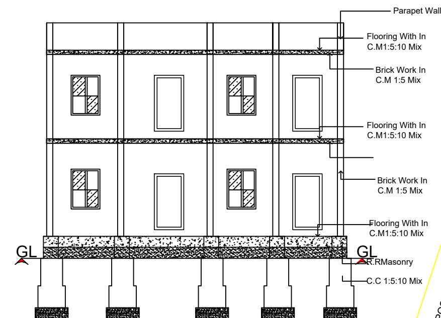
SECTION @ AA' FOUNDATION DETAIL DESIGNED
