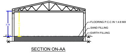
SECTION ON-AA
