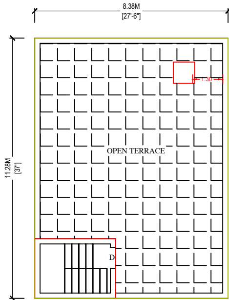
PRO.TERRACE FLOOR PLAN
