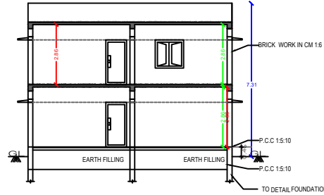
SECTION "A-B"
