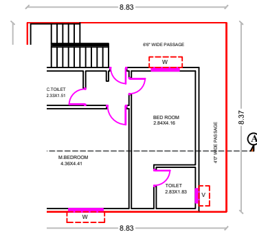
PRO.FIRTS FLOOR PLAN
