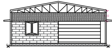
FRONT ELEVATION
