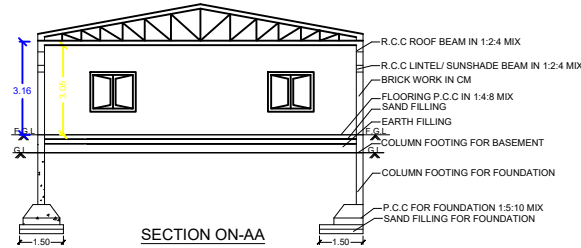
SECTION ON-AA
