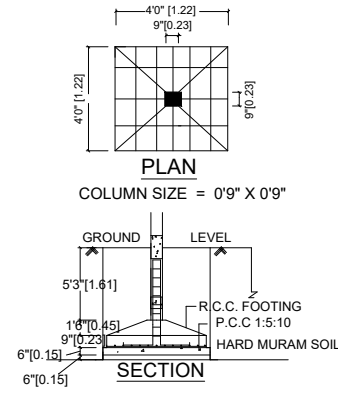
FOUNDATION DETAILS
