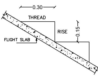
STAIRCASE DETAILS
