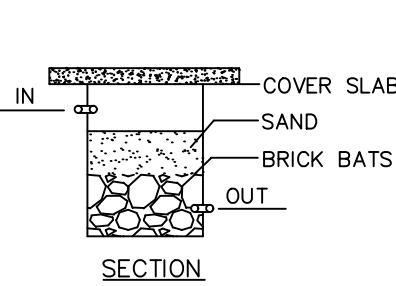
RAINWATER HARVEST
