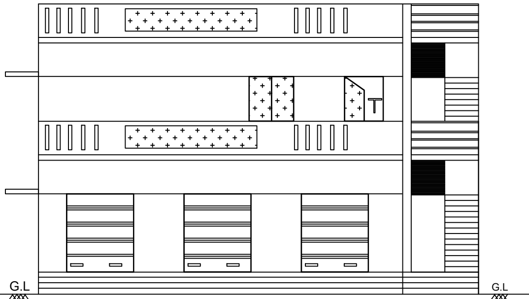
FRONT ELEVATION
