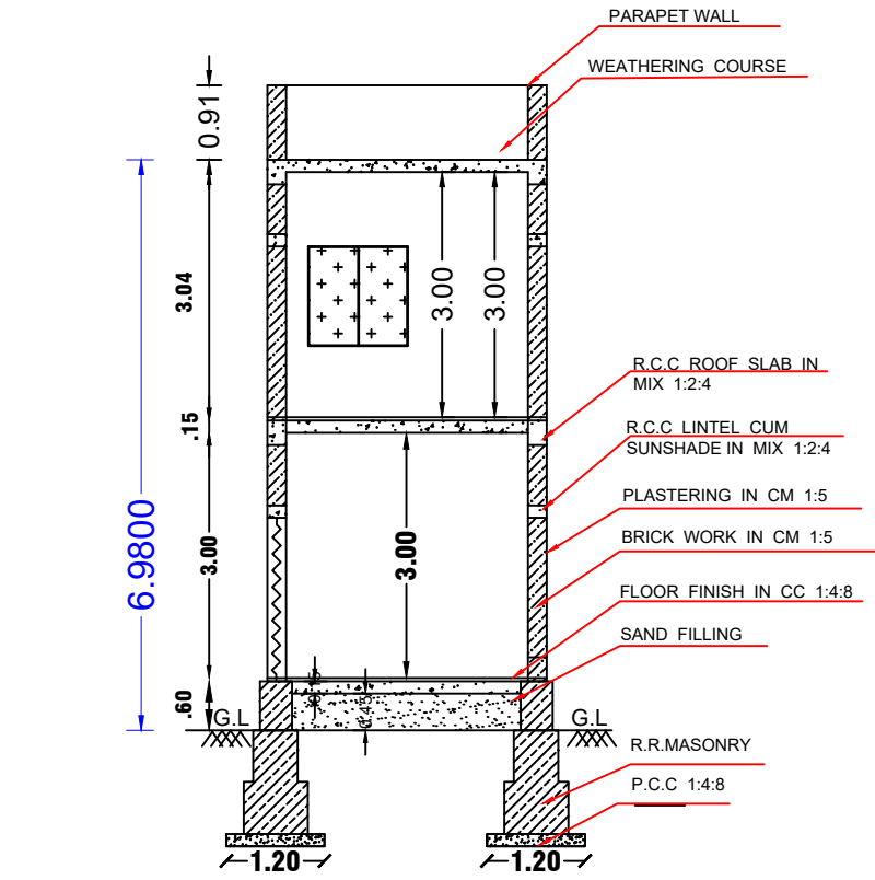
SECTION ON-"AB"
