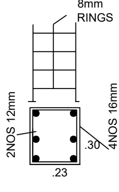
COLUMN DETAILS
