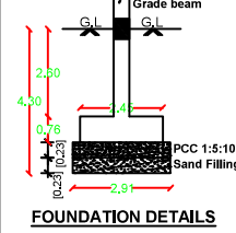
FOUNDATION DETAILS
