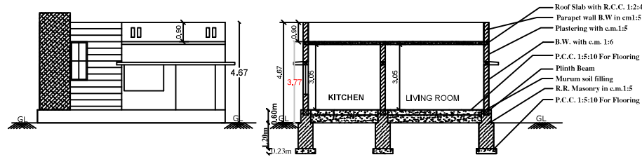
FRONT ELEVATION
