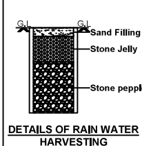
BORE WELL
