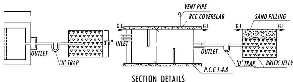
SEPTIC TANK AND DISPERSION TRENCH DETAILS
